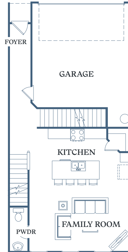
1 ST FLOOR – 715 SF
